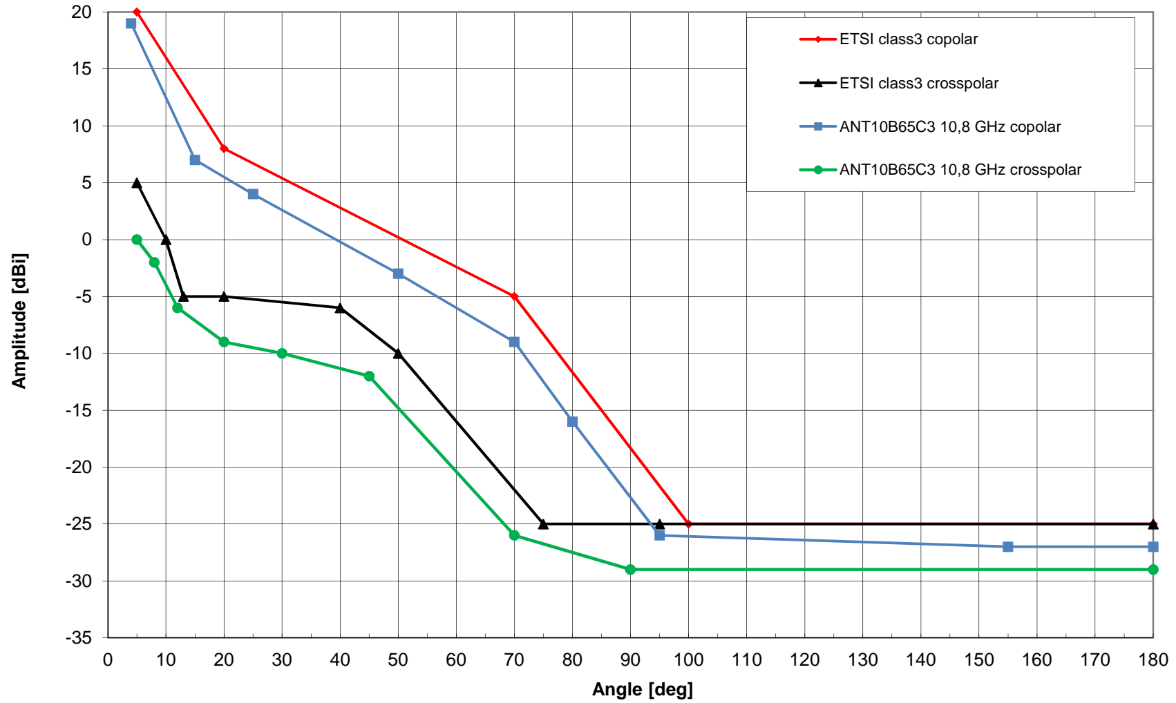
Radiation pattern ANT10B65C3 10,8 GHz, max. gain 34,8 dBi
