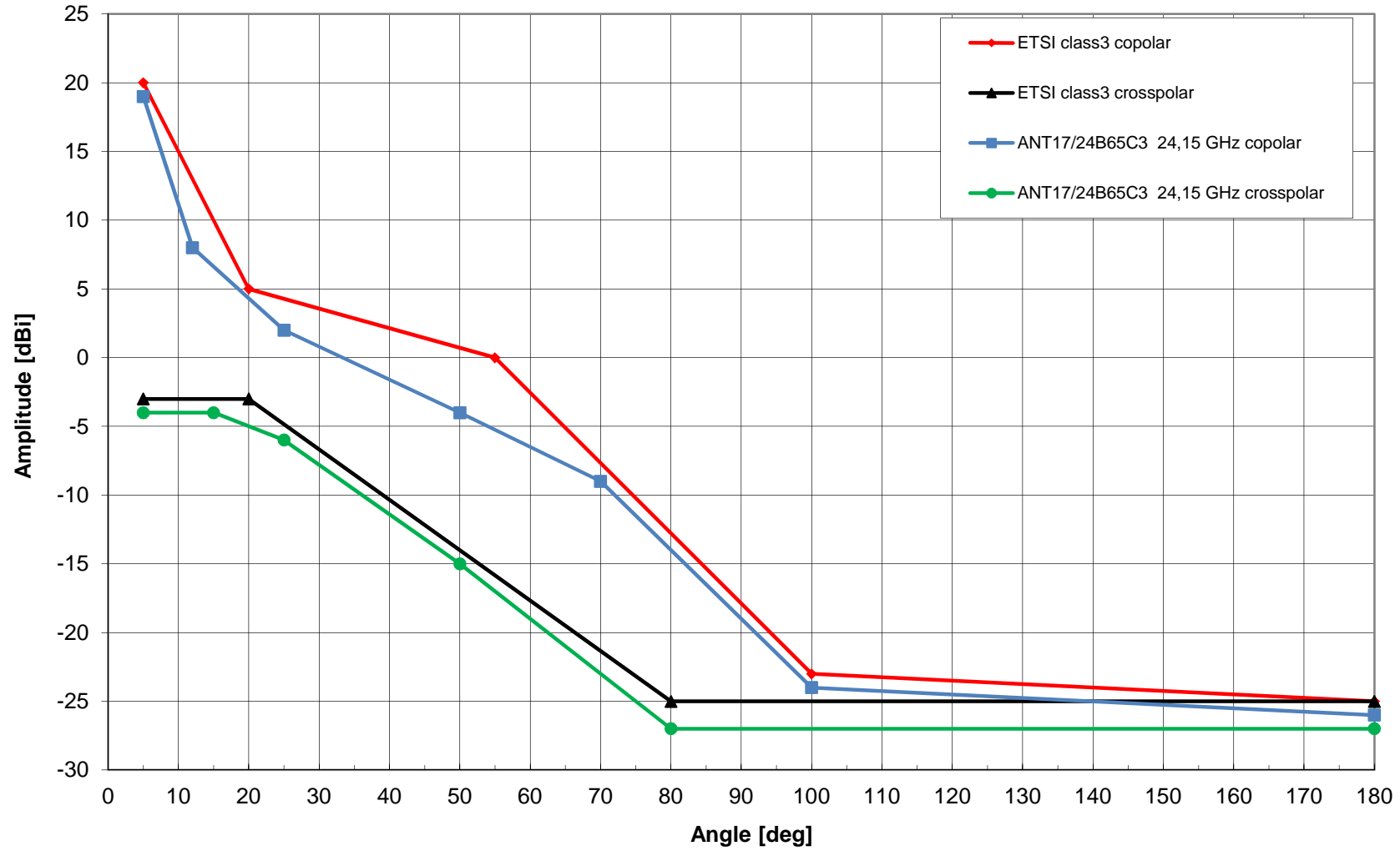
Radiation pattern ANT17/24B65C3 24,15 GHz, max. gain 41,0 dBi
