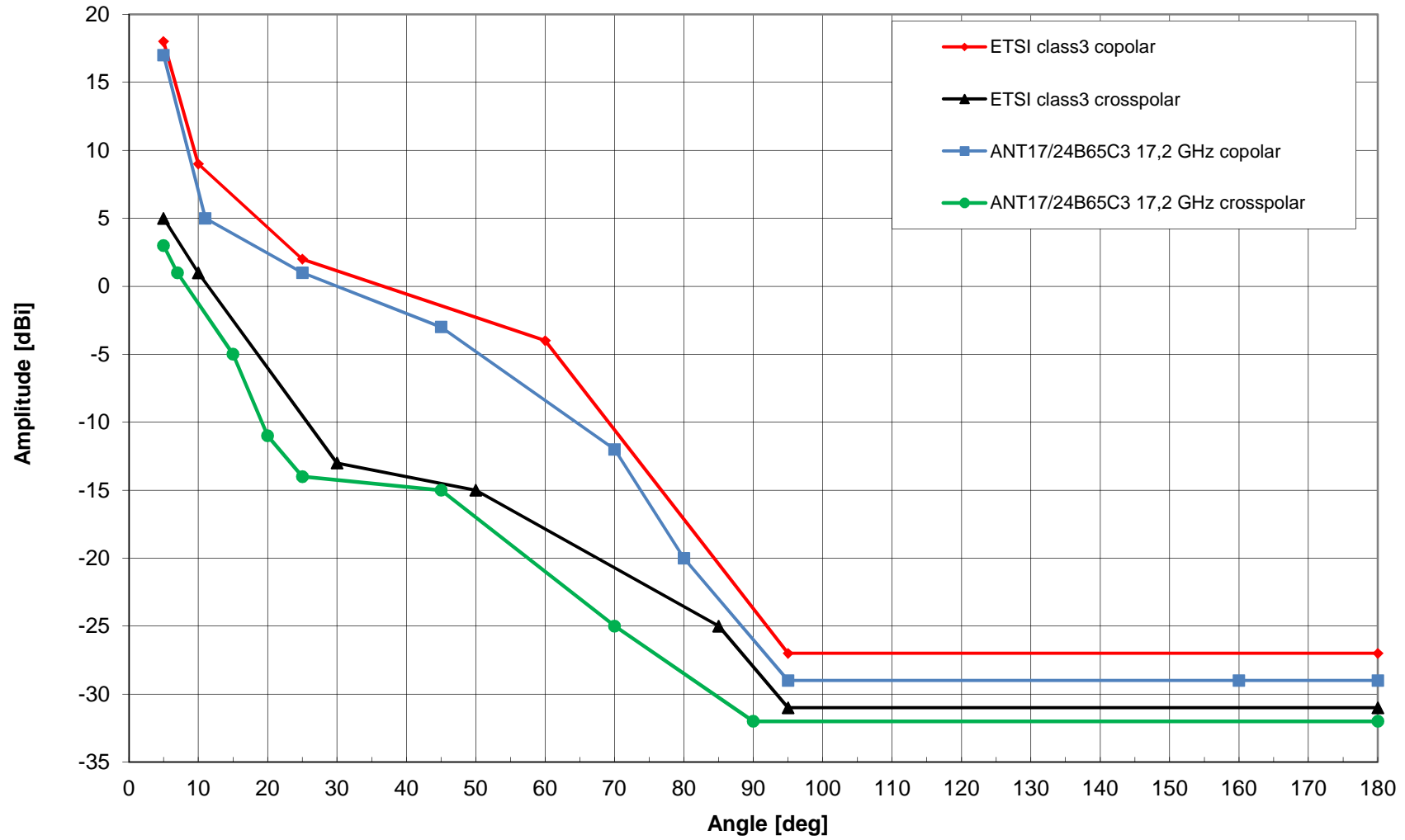
Radiation pattern ANT17/24B65C3 17,2 GHz, max. gain 38,0 dBi
